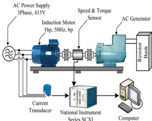
Fig .1: Shows the Fault Detection Setup
