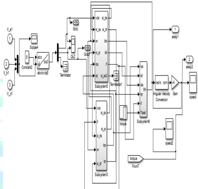
Fig. 4: Shows the Mathematical Model of Induction Motor
