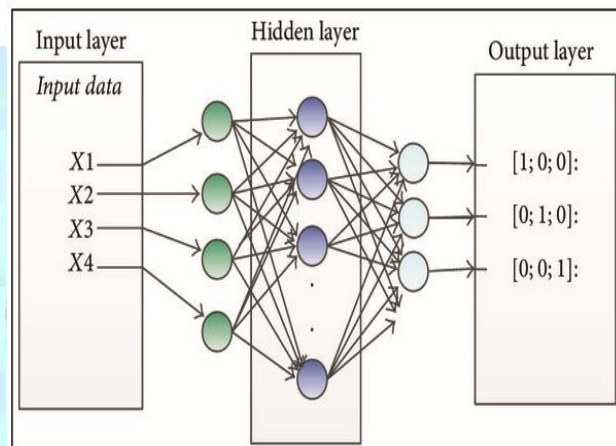
Fig. 3: ANN based Motor Rotor Fault Detection
